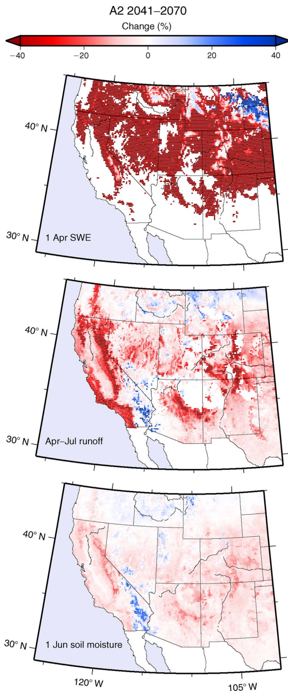
FIG. 2. Projected changes in snow (snow water equivalent, SWE), runoff, and soil moisture, as percent change in 2041–2070 from 1971–2000 conditions, under continued increases in greenhouse-gas emissions (A2 scenario; Cayan et al. 2013).
